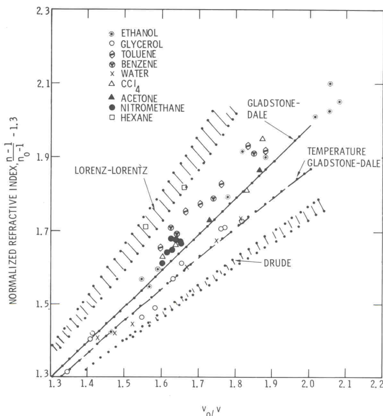
Fig. 5.2. The collected data on index of refraction of shock-loaded fluids give little support to a universal model to describe the effect of compression on refractive index. (After Kormer [68K5].)
